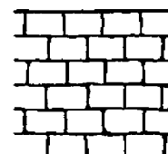
COBBLEBRICK AVERAGE BRICK SIZE: 5 1/2" X 8 1/2" ROLL WIDTH: 37" JOINT WIDTH: 1/2" - 3/4"
