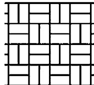
BASKET WEAVE BRICK SIZE: 3 1/2" X 7 3/4" ROLL WIDTH: 33 1/2" JOINT WIDTH: 1/2"
