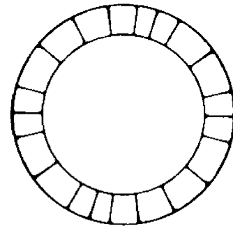
COBBLE CIRCLE RING DIAMETER 7' 2" JOINT WIDTH: 1/2"
