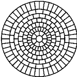
BRICK ROSETTE DIAMETER: 5' 5 1/4" JOINT WIDTH: 1/2"
