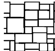
ASHLAR TILE LARGEST TILE SIZE: 12 1/4" X 11 1/4" ROLL WIDTH: 37" JOINT WIDTH: 1/2" - 1"
