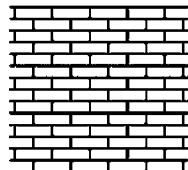
FACE BRICK BRICK SIZE: 2 3/16" X 7 7/8" ROLL WIDTH: 36 7/8" JOINT WIDTH: 7/16"
