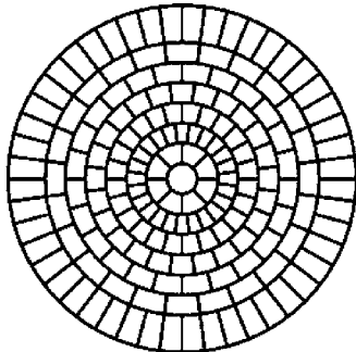
LARGE BRICK ROSETTE DIAMETER: 7' 2" JOINT WIDTH: 7/8"
