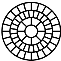
SMALL BRICK ROSETTE DIAMETER: 2' 11 1/2" JOINT WIDTH: 1/2"
