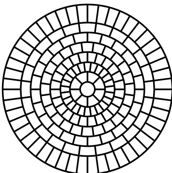
LARGE BRICK ROSETTE DIAMETER: 7' 2" JOINT WIDTH: 7/8"
