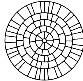
COBBLE CIRCLE DIAMETER: 5' 5" JOINT WIDTH: 1/2"
