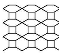
MEDITERRANEAN OCTAGON: 21" X 13 7/8" ROLL WIDTH: 32" JOINT WIDTH: 1/2"
