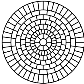
BRICK ROSETTE DIAMETER: 5' 5 1/4" JOINT WIDTH: 1/2"
